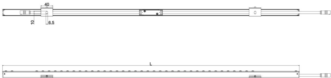
@Screw-in Bracket (b), L=1000/500/300mm
