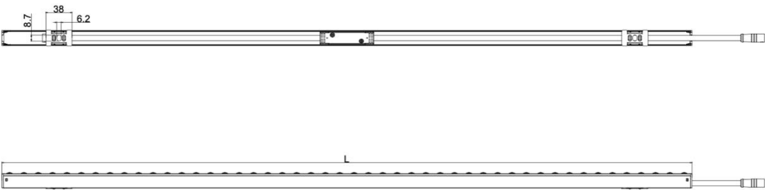
@Clip Bracket (a), L=1000/500/300mm
