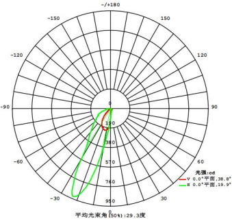
Beam Angle (FWHM): T4S1L
