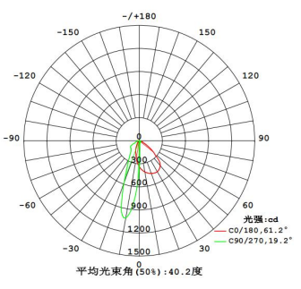
Beam Angle (FWHM): T4S2R
