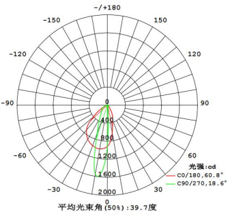
Beam Angle (FWHM): T4S2L
