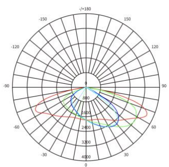
Beam Angle (FWHM): T3M
