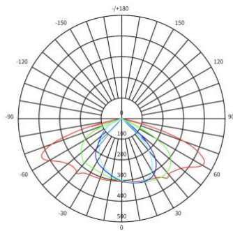
Beam Angle (FWHM): T2M
